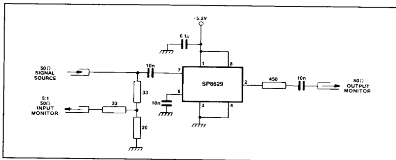
Fig.5 Test circuit
