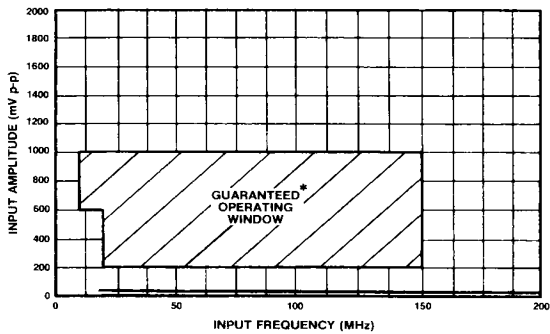
Fig.3 Typical input characteristics SP8629
