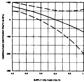
CENTER FREQUENCY COEFFICIENT TEMPERATURE (MEAN AND S.D.)
