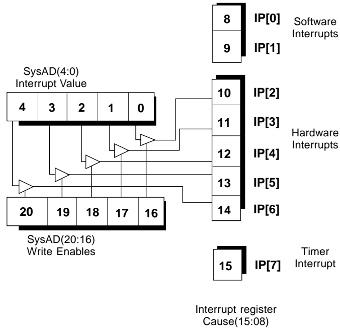
Figure 6-5 Hardware Interrupts
