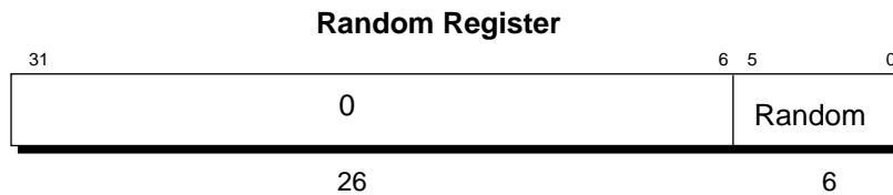
Figure 13-2 Random Register
