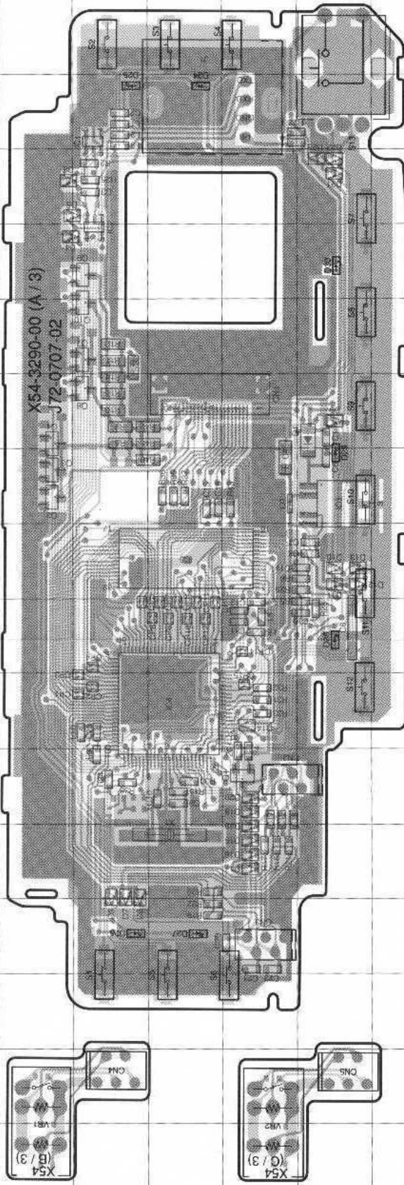
PANEL UNIT (X54-3290-00) Foil side view
